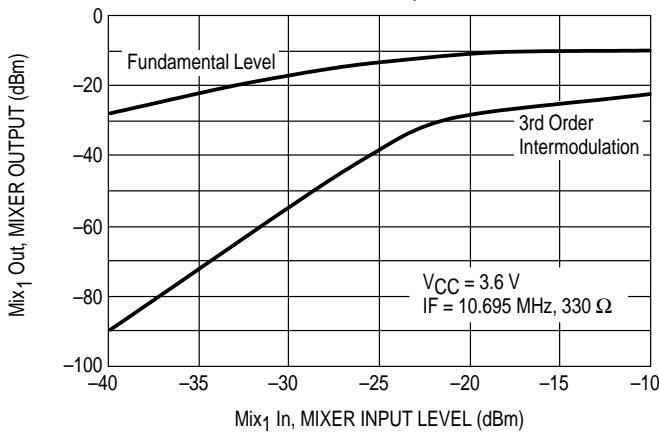
Figure 19. First Mixer Output Level and Intermodulation, IP3_bit = 0
